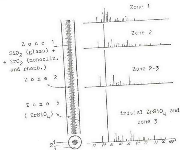
Fig. 3. Shocked powder of ZrSiO_4 .
